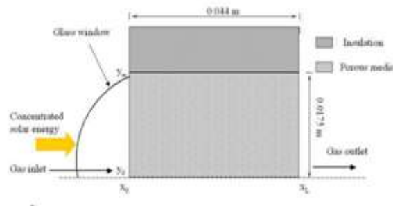
Figure 3 Cross-section sketch of the solar reactor
