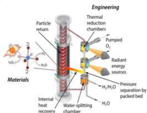
Figure1 Solar Thermochemical Reactor for Hydrogen
