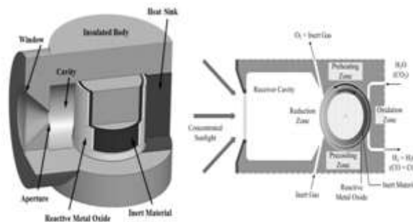
Figure 2 Reactor for solar-driven non-stoichiometric redox cycling of a metal oxide
